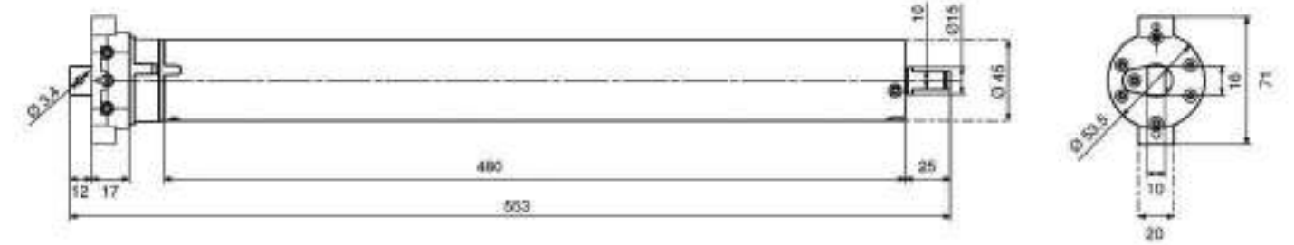
TEKNİK DETAY TABLOSU TECHNICAL DETAIL CHART
