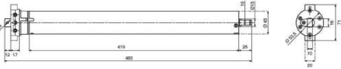
TEKNİK DETAY TABLOSU TECHNICAL DETAIL CHART
